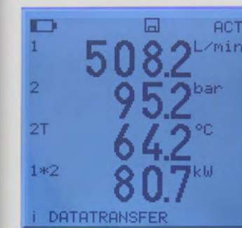
HPM4030 data logging 3 readings + calculated power
