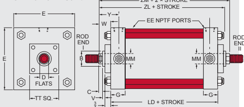
8 Thru 16" Mount
